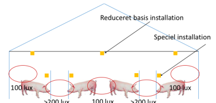
OPTIMAL LIGHT INSTALLATION
